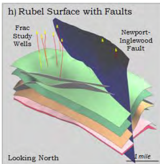
Figure 2-8H Rubel Surface with Faults
