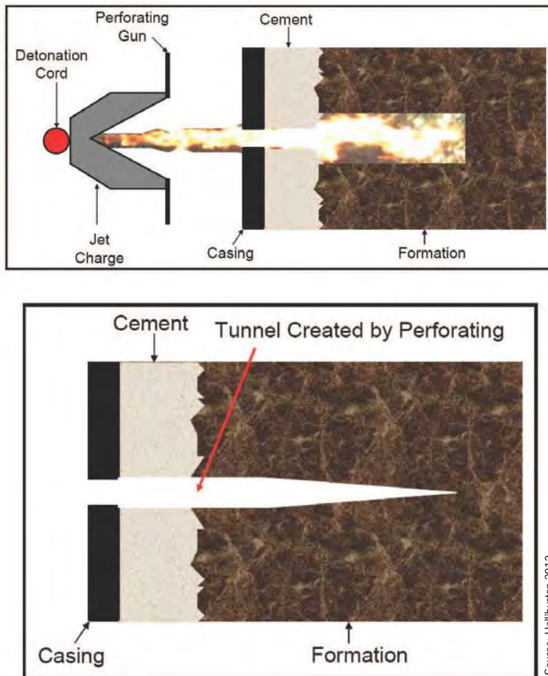
Figure 3-2 Perforation Process
