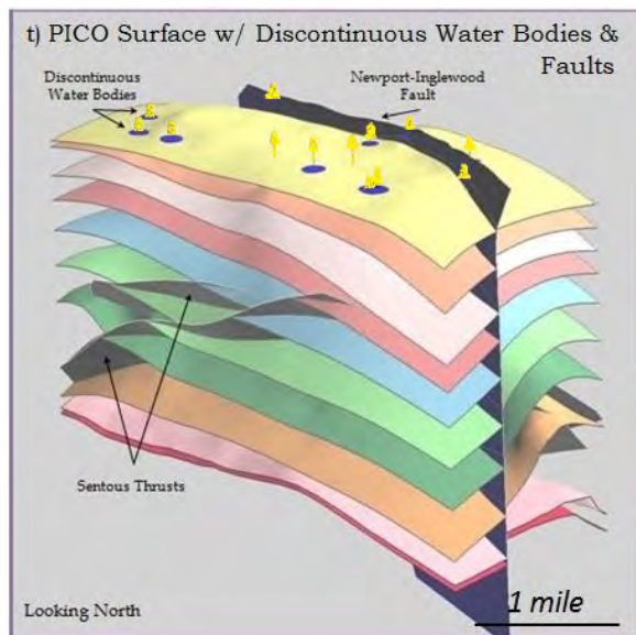
Figure 2-8T PICO Surface w/ Discontinuous Water Bodies & Faults
