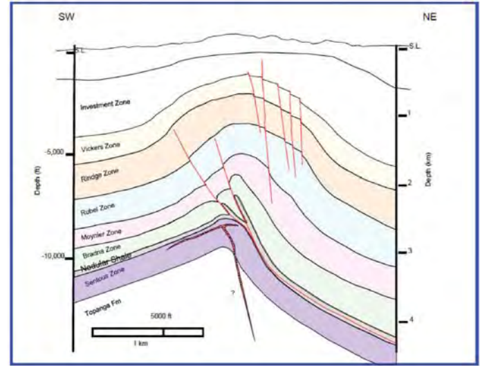
Schematic cross section of Inglewood Field, northern portion (Elliott 2009)
