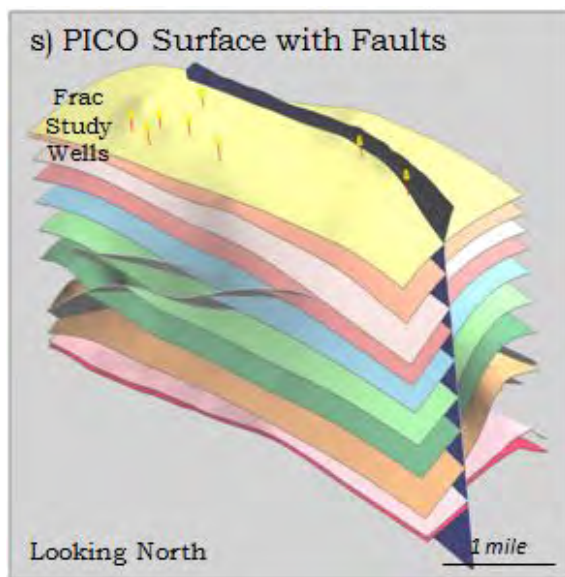
Figure 2-8S PICO Surface with Faults
