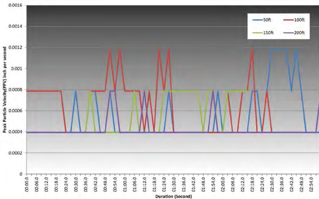
Figure 4-10B Ground Vibration Level Measurements from High-Volume Hydraulic Fracture at VIC1-635
