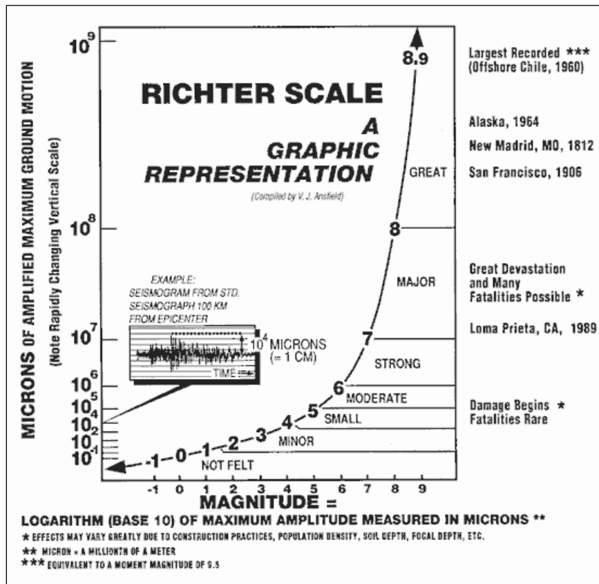
Figure 3-7 Graphical Representation of Seismic Events as Recorded on the Richter Scale
