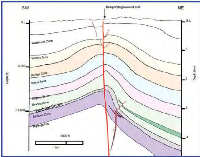
Schematic cross section of Inglewood Field, southern portion (Elliott 2009)
