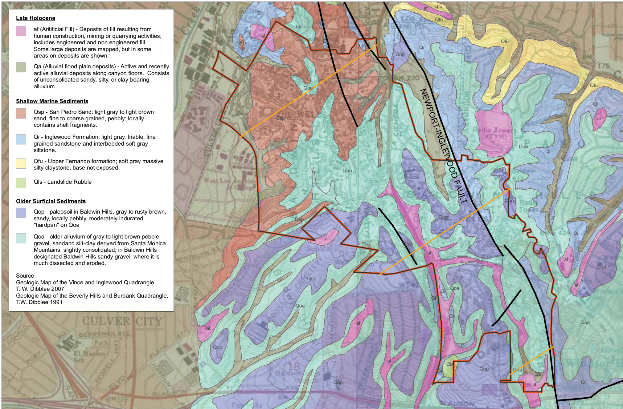
Figure 2-6 Geologic Formations Present at the Inglewood Oil Field and Vicinity 10 | 01 | 12
